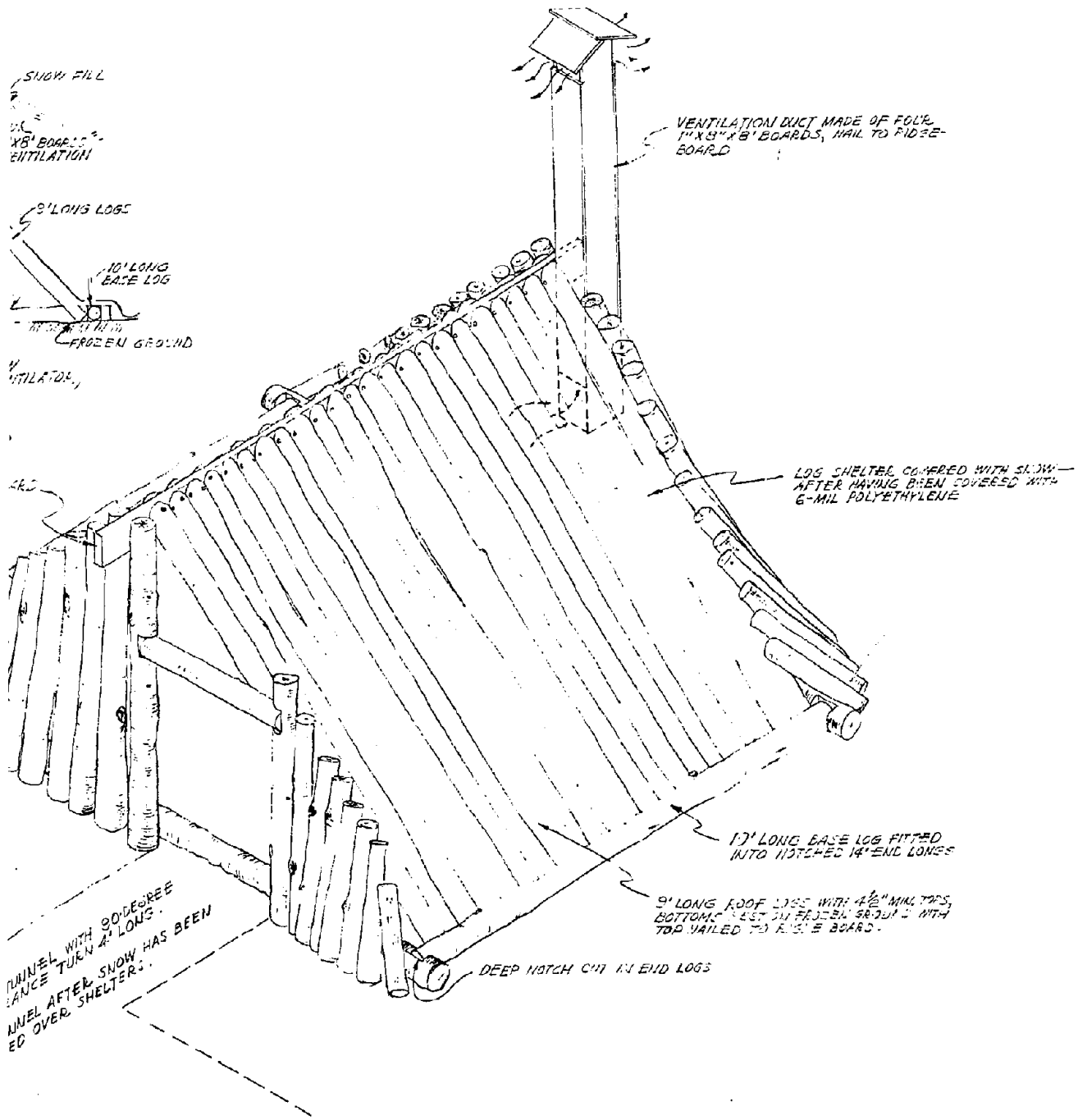
Fig. A-4.2. Two-Family A-Frame Pole Shelter, Frozen Ground Version.
